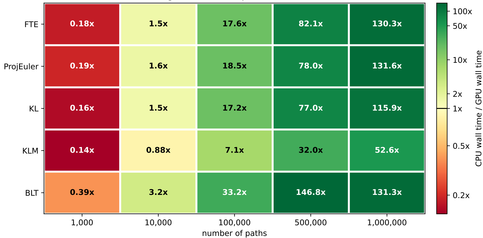
GPU acceleration by scheme and workload regime B, 512 steps, FP64, P100
