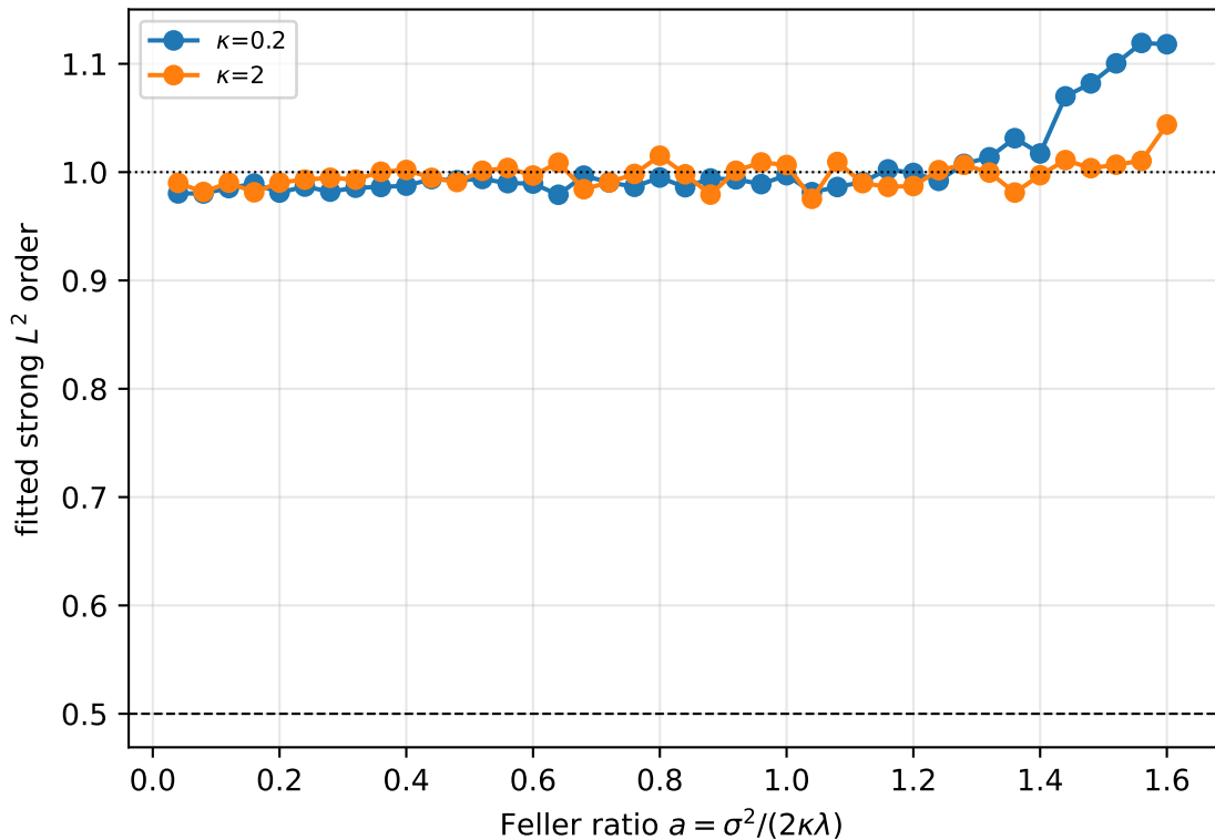
KLM backstopped adaptive scheme: observed order across a
