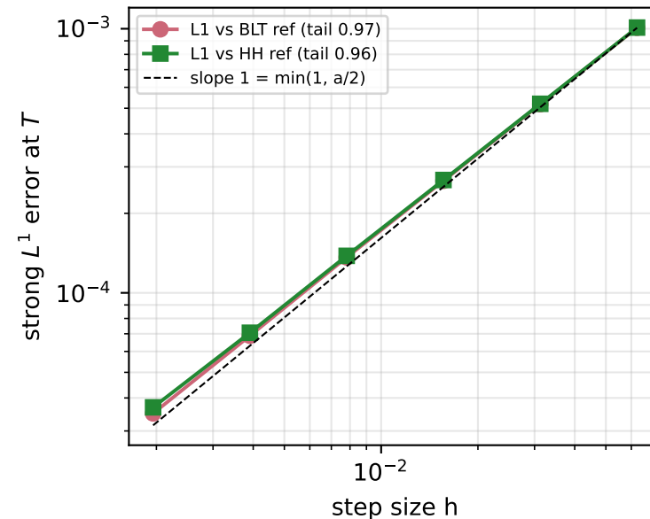
Regime C: a = \delta = 2
