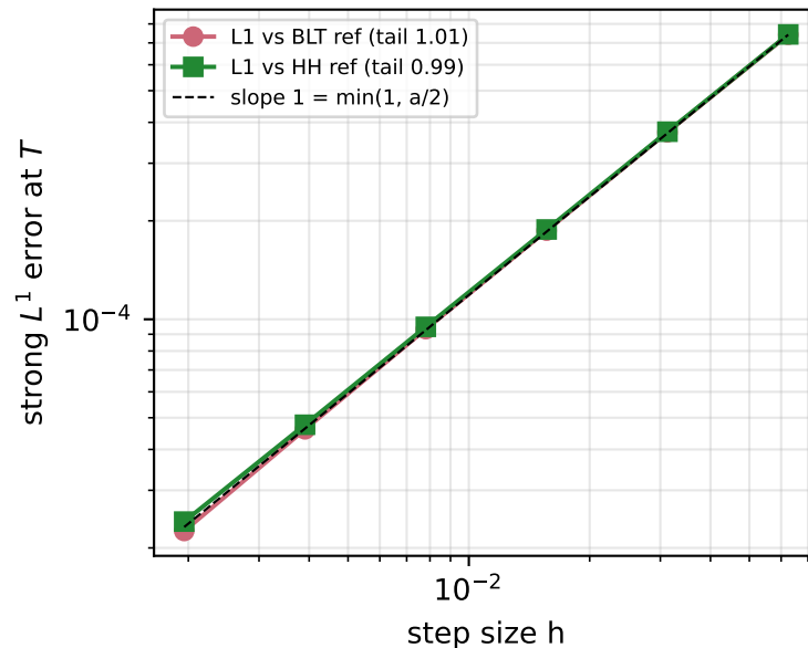
Regime B: a = \delta = 4
