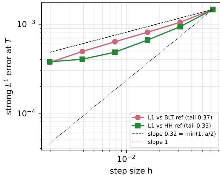
Regime D: a = \delta = 0.64
