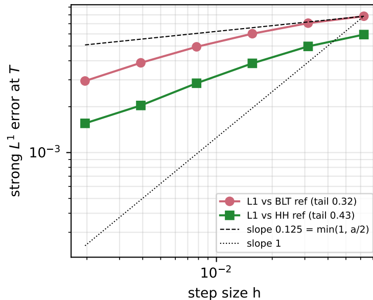
Regime E: a = \delta = 0.25
