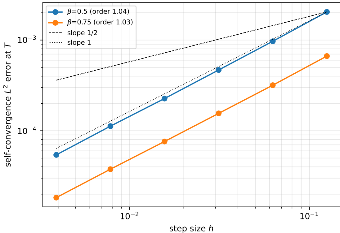
CEV projected Lamperti scheme, regime B ( \sigma=0.2 ), 20000 paths
