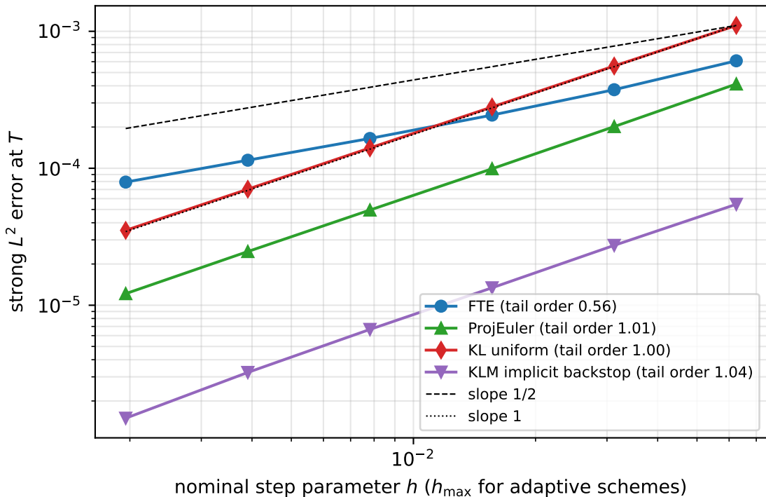
Regime A: \sigma = 0.1 , 20000 paths HH fine reference at 32768 steps
