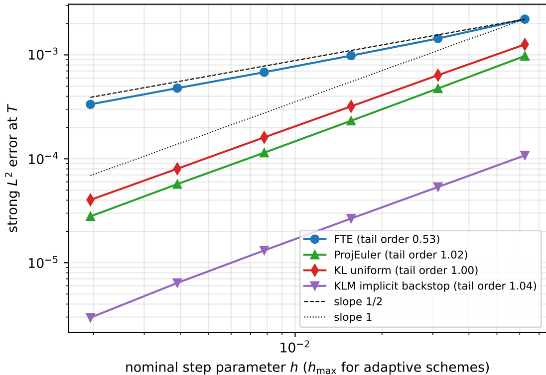
Regime B: \sigma = 0.2 , 20000 paths, HH fine reference at 32768 step
