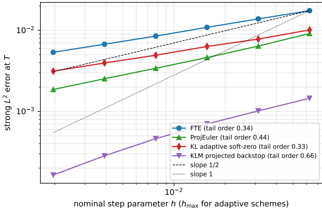
Regime D: \sigma = 0.5 , 20000 paths HH fine reference at 32768 steps
