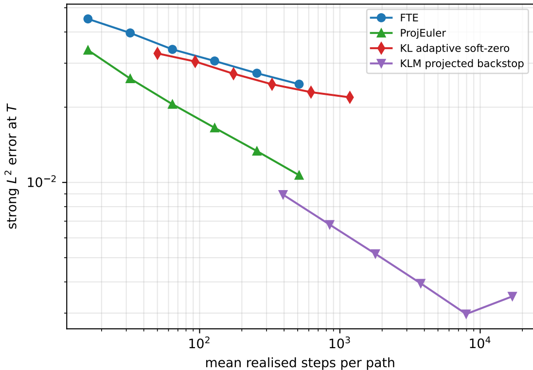
Regime E: cost-normalised view, \sigma = 0.8 , 20000 paths, HH reference
