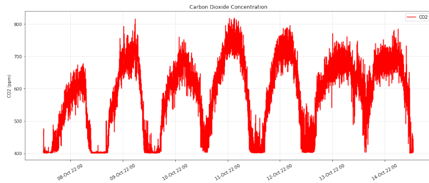
Figure 6.10: CO 2 Profile
