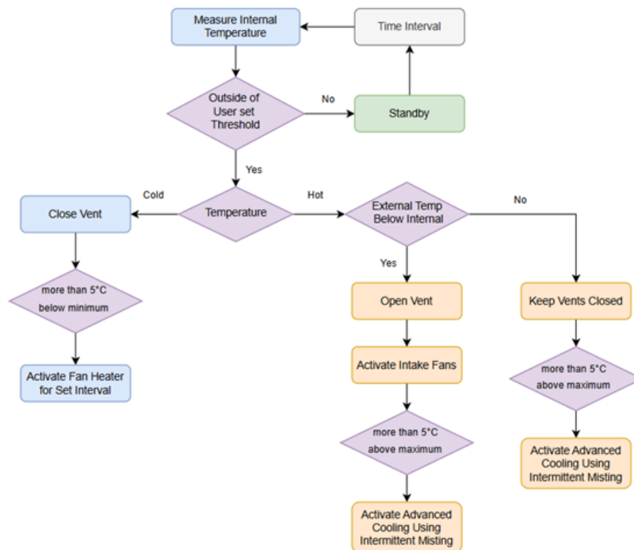
Figure 5.3: Temperature control
