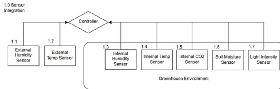
Figure 3.2: Sensor Physical Decomposition
