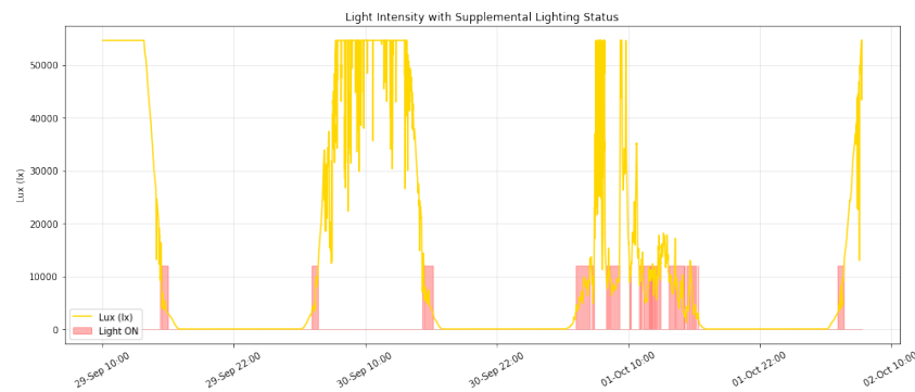
Figure 6.12: Lux Profile
