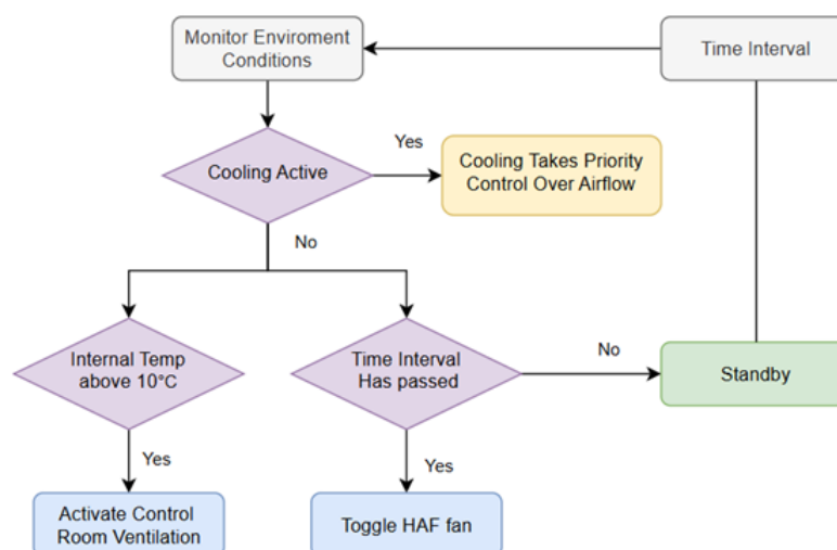
Figure 5.4: Airflow control
