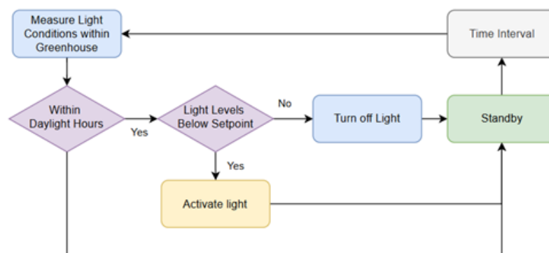
Figure 5.6: Light control
