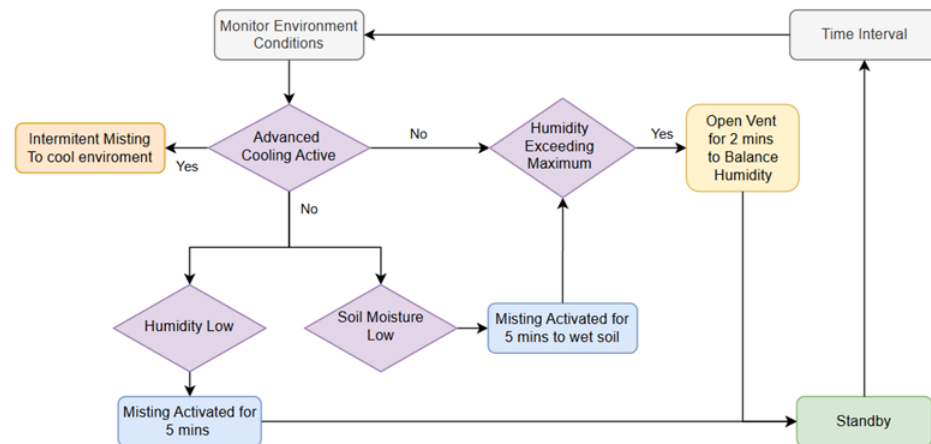
Figure 5.5: Irrigation control
