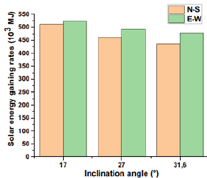
Figure 2.3: Solar radiation gain vs inclination angles (Mellalou et al. , 2022).
