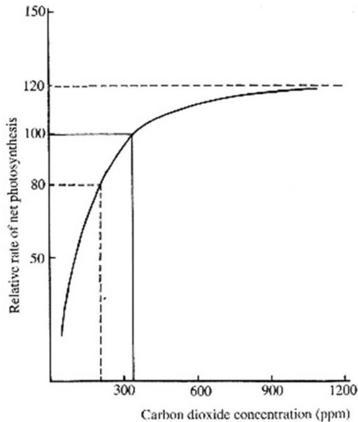
Figure 2.1: Effect of CO 2 concentration on photosynthesis rate. (UC Agriculture and Natural Resources, n.d.).
