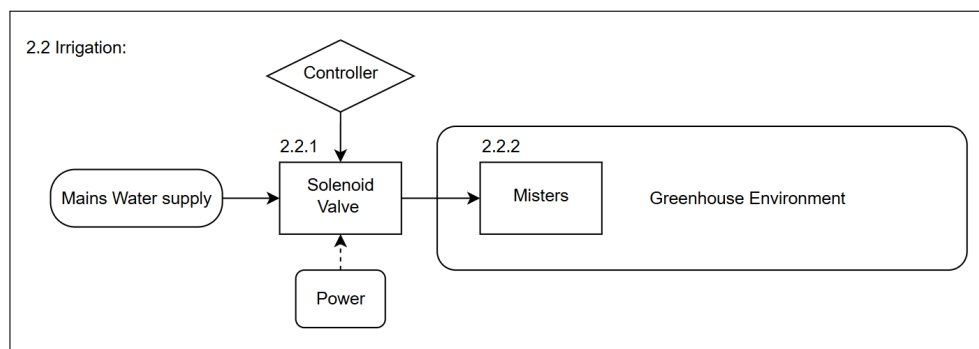
Figure 3.4: Irrigation Physical Decomposition
