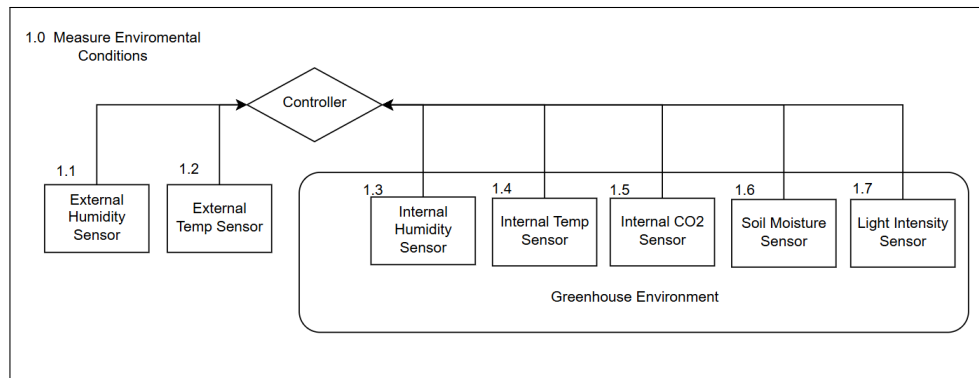
Figure 3.2: Environmental monitoring Physical Decomposition
