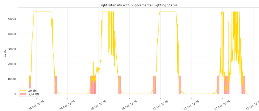
Figure 6.11: Lux Profile
