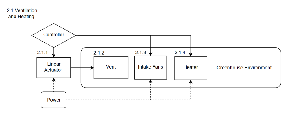
Figure 3.3: Ventilation and Heating Actuation Physical Decomposition
