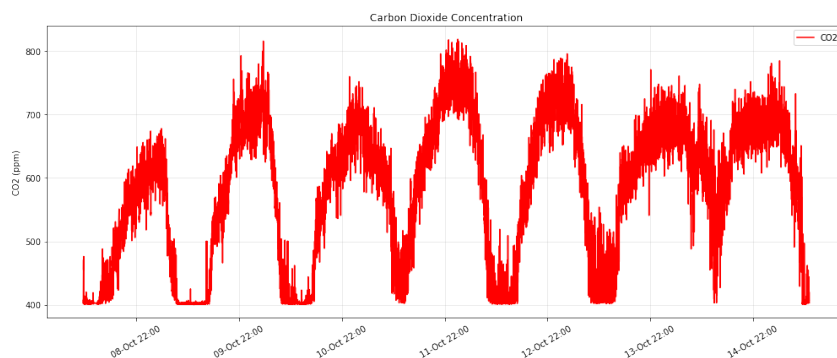
Figure 6.10: CO 2 Profile
