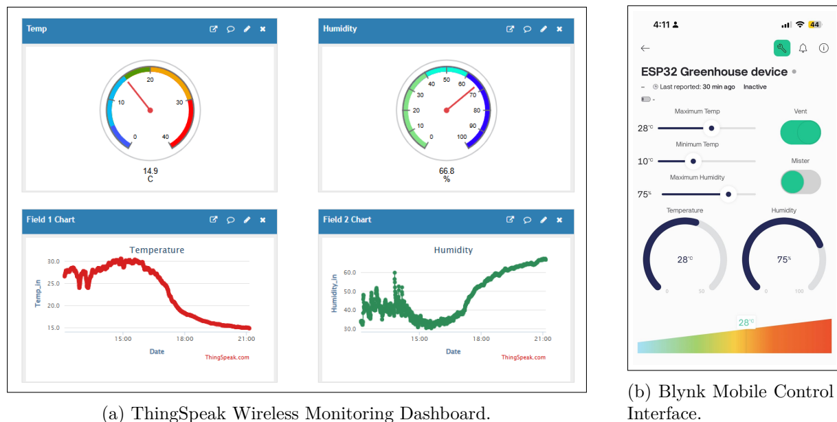
Figure 6.6: Remote monitoring and control interfaces
