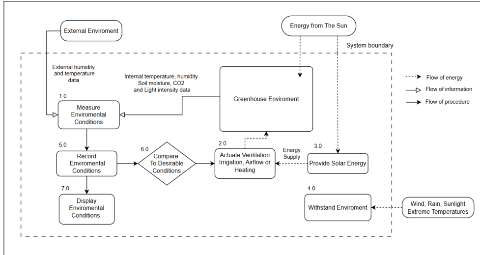
Figure 3.1: Functional decomposition
