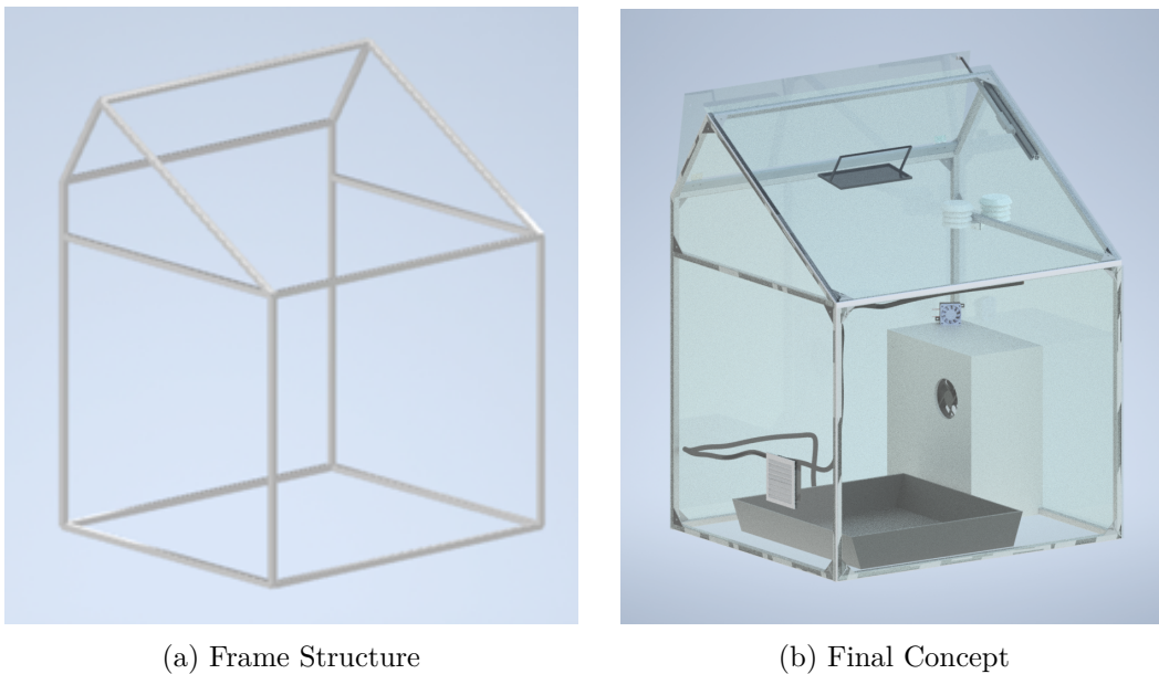
Figure 4.1: Detailed Design
