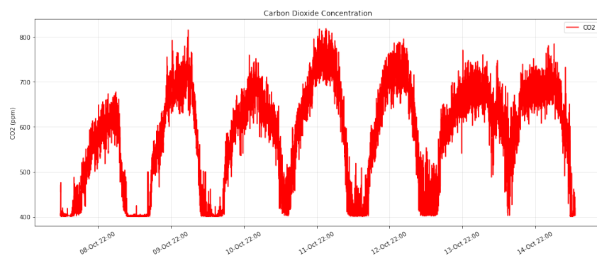
Figure 6.11: CO 2 Profile
