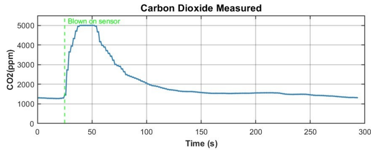
Figure 6.4: CO 2 sensor response to rapid change in concentration.
