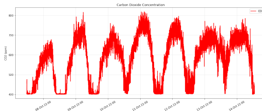
Figure 6.11: CO 2 Profile
