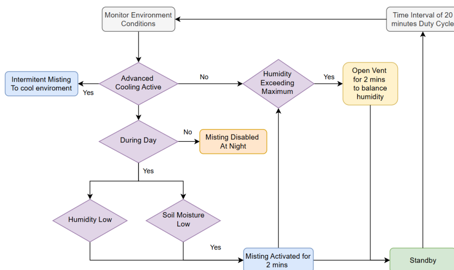
Figure B.3: Irrigation control
