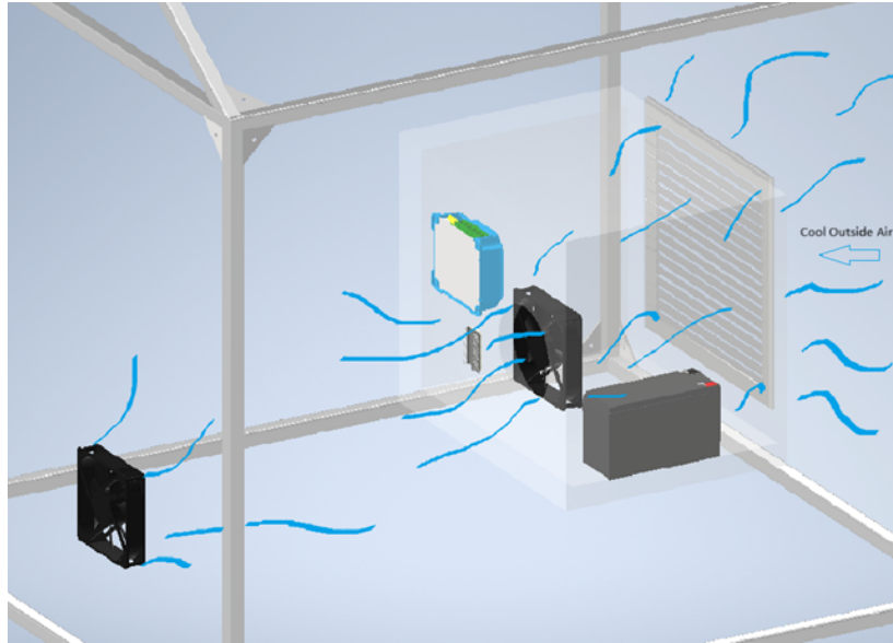
Figure 4.5: Air Intake
