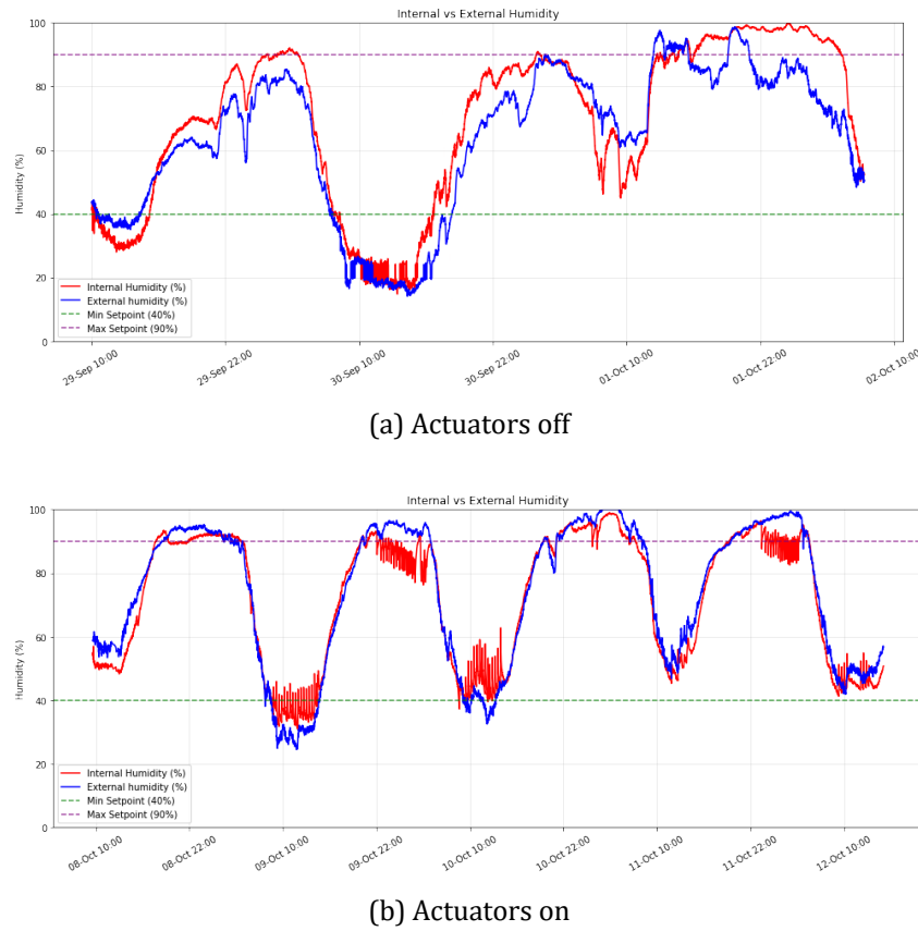
Figure 6.9: Internal vs. external humidity profiles for the greenhouse with (a) actuators off and (b) actuators on.
