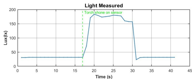
Figure 6.3: BH1750 light sensor response to torch illumination and return to ambient lighting.
