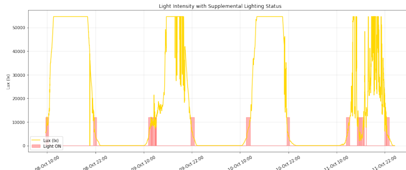
Figure 6.12: Lux Profile
