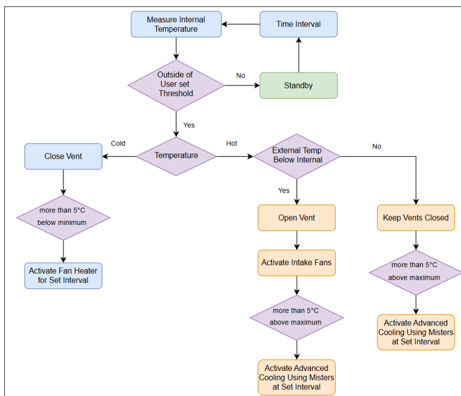
Figure C.1: Temperature control
