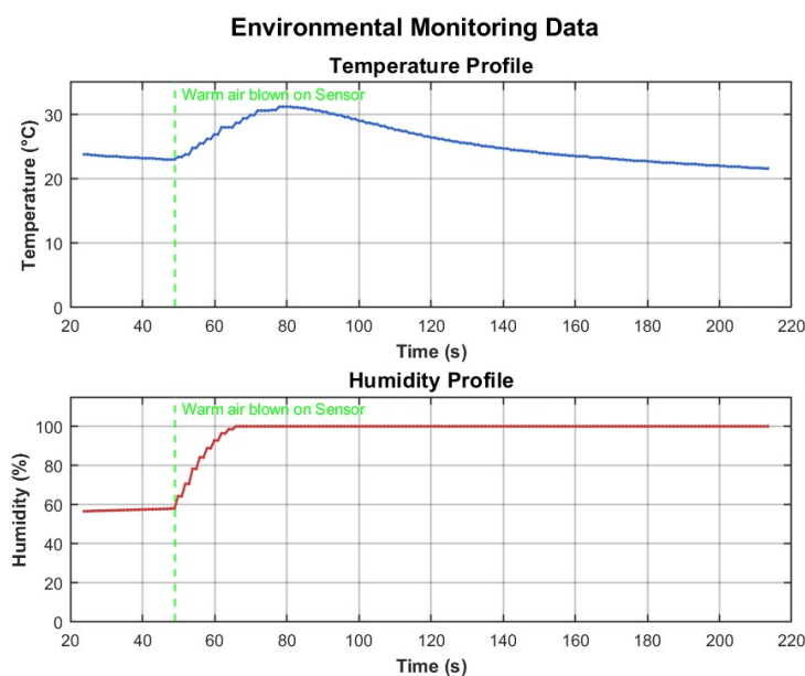
Figure 6.2: DHT22 response to applied warm air (temperature and humidity vs. time).
