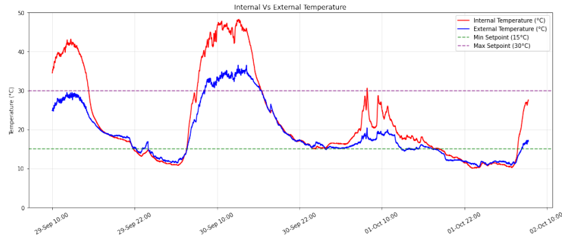
(a) Temperature profile with Actuators off
