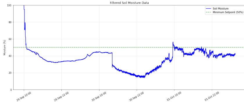
(a) Soil Moisture profile with Actuators off
