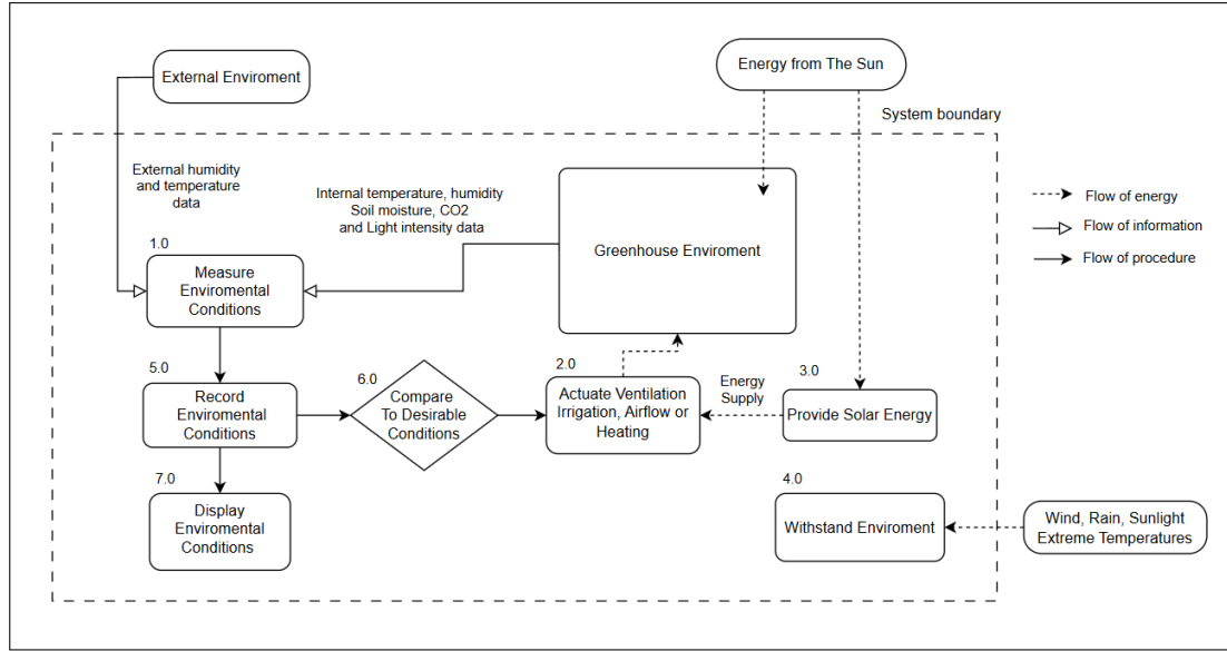
Figure 3.1: Functional decomposition
