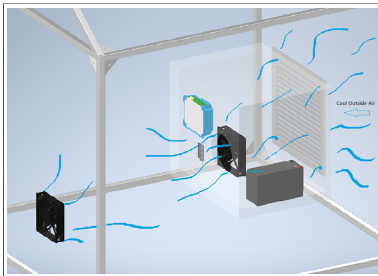
Figure 4.3: Air Intake
