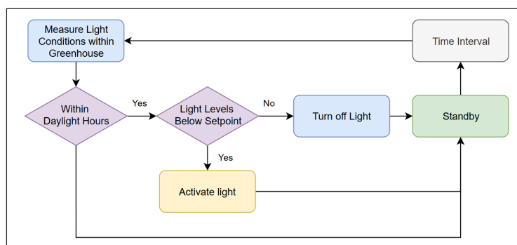
Figure C.4: Light control
