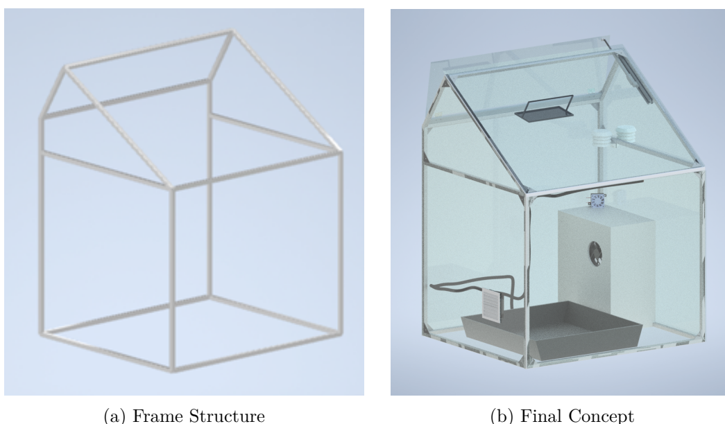
Figure 4.1: Detailed Design
