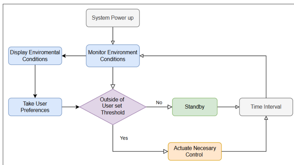
Figure 5.2: Principal Control Flowchart
