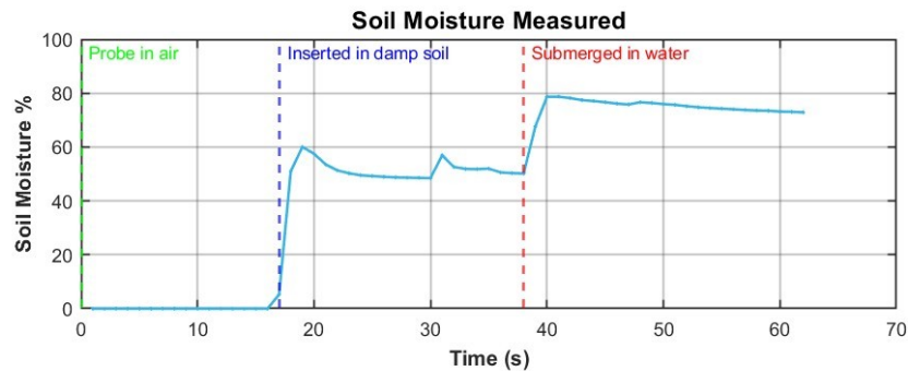
Figure 6.2: Soil moisture sensor response in open air, damp soil, and submerged in water.
