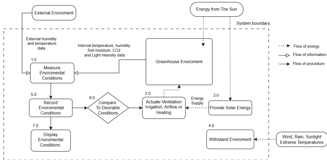
Figure 3.1: Functional decomposition
