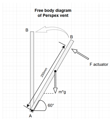
Figure 4.4: Free body diagram of Vent Mechanism
