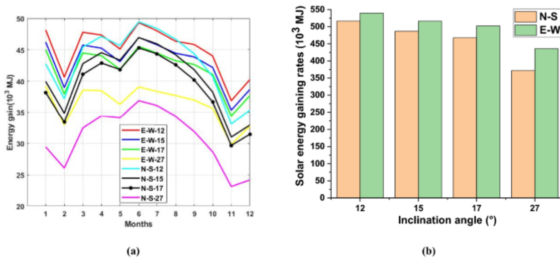
Figure 2.3: Solar radiation gain vs inclination angles (Mellalou et al. , 2022).
