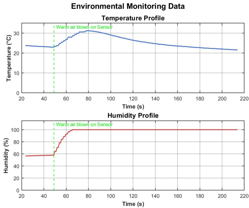
Figure 6.1: DHT22 response to applied warm air (temperature and humidity vs. time).
