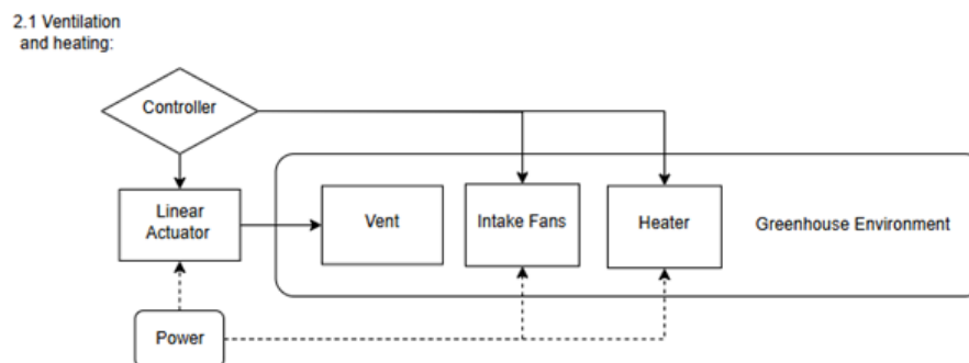
Figure 3.3: Ventilation Physical Decomposition
