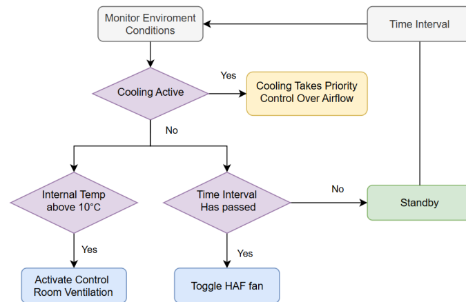
Figure B.2: Airflow control
