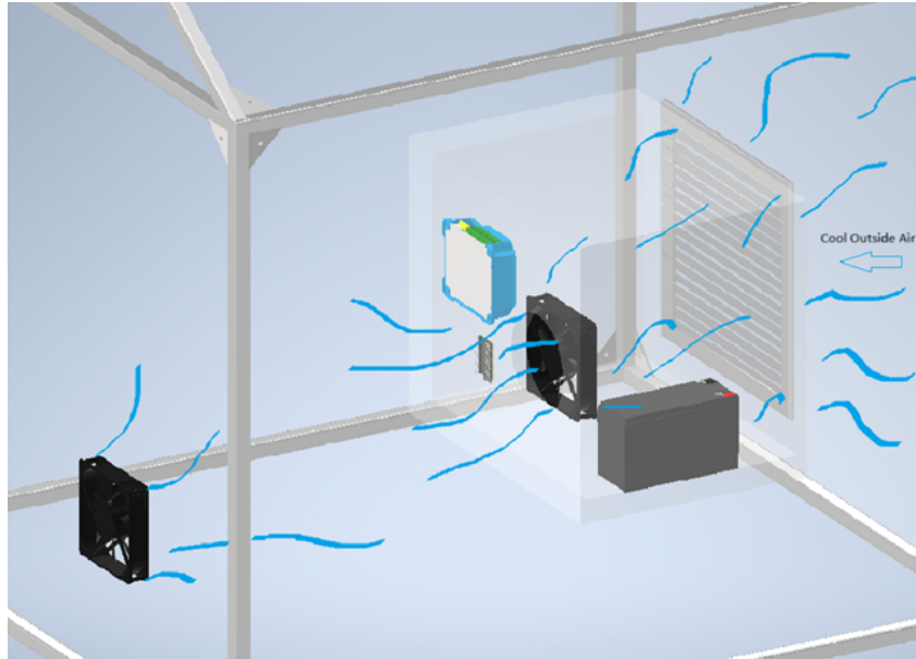
Figure 4.5: Air Intake
