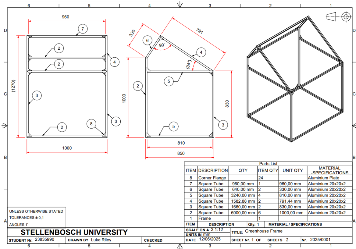
Figure E.1: Engineering Drawing
