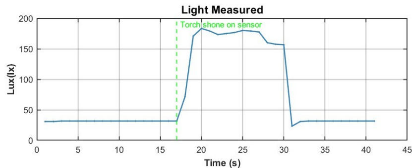
Figure 6.3: BH1750 light sensor response to torch illumination and return to ambient room lighting.
