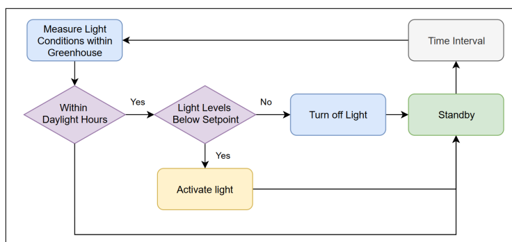
Figure B.4: Light control
