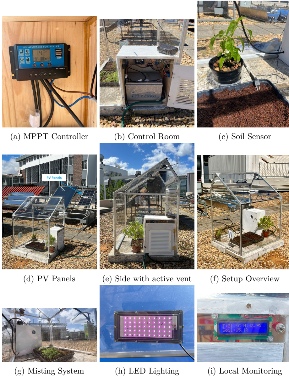
Figure G.1: Overview of greenhouse hardware components and setup.
