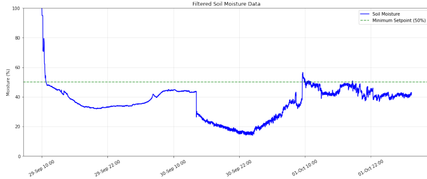
(a) Actuators off
