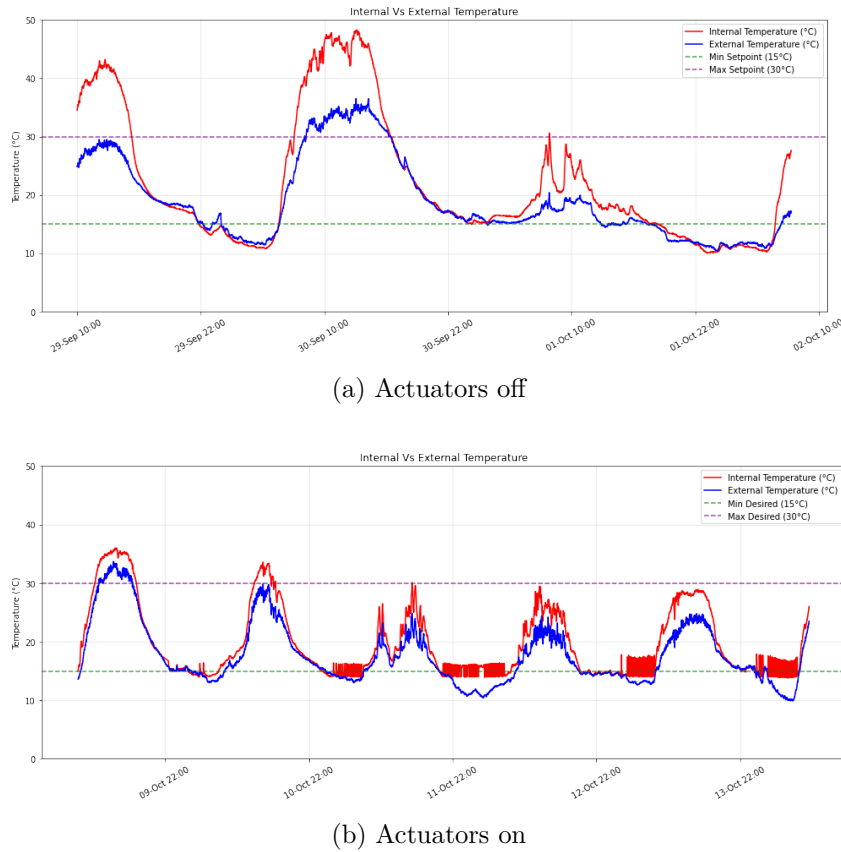
Figure 6.7: Internal vs. external temperature profiles for the greenhouse with (a) Actuators off and (b) Actuators on.
