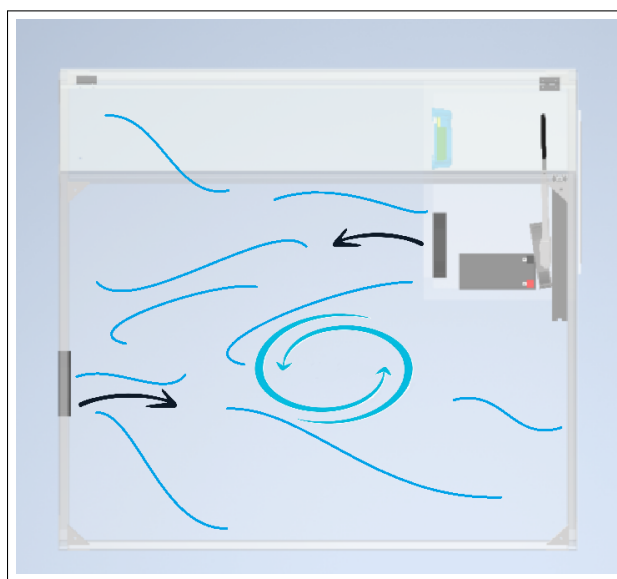
Figure 4.4: Air circulation
