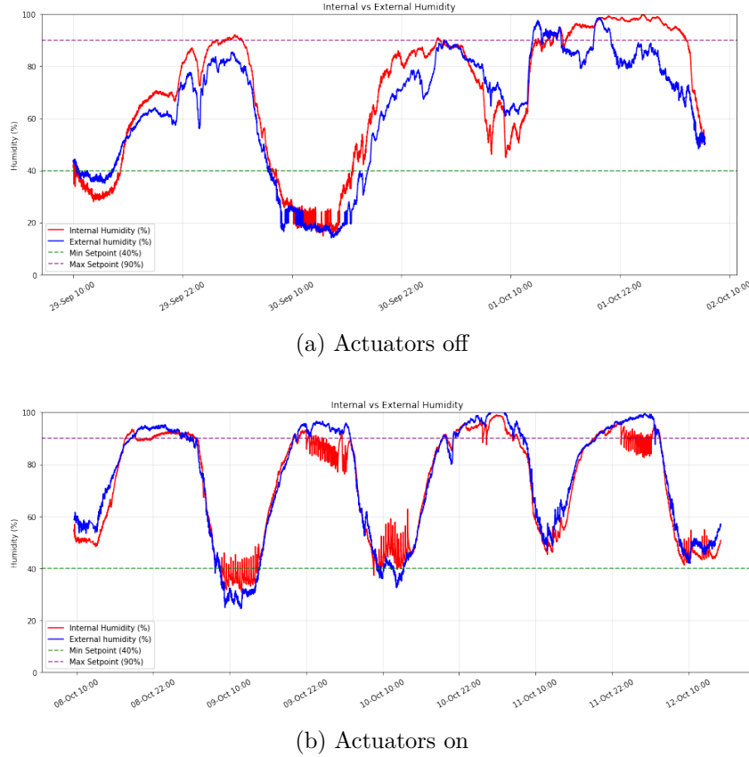
Figure 6.8: Internal vs. external humidity profiles for the greenhouse with (a) actuators off and (b) actuators on.
