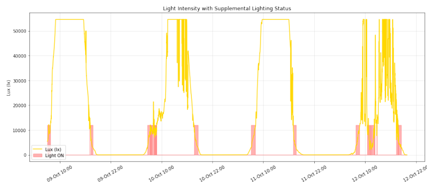
Figure 6.11: Lux Profile
