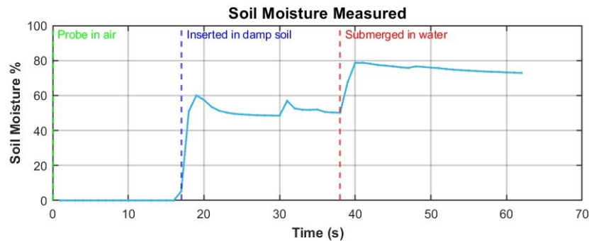
Figure 9.2: Soil moisture sensor response in open air, damp soil, and submerged in water.
