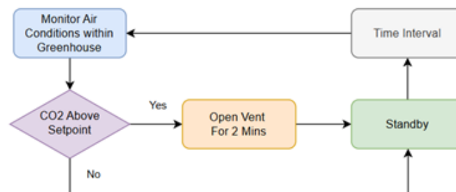
Figure 8.7: Air quality Control
