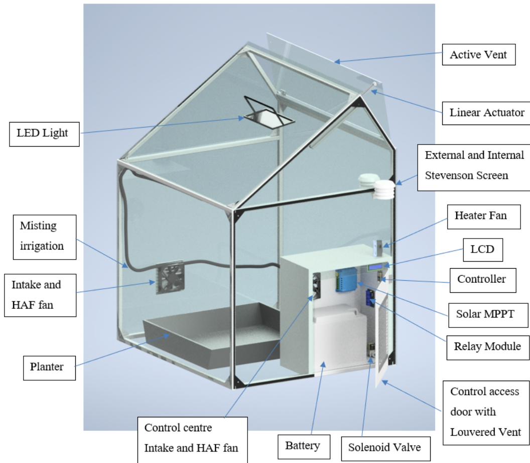
Figure 7.2: Final Concept Definition
