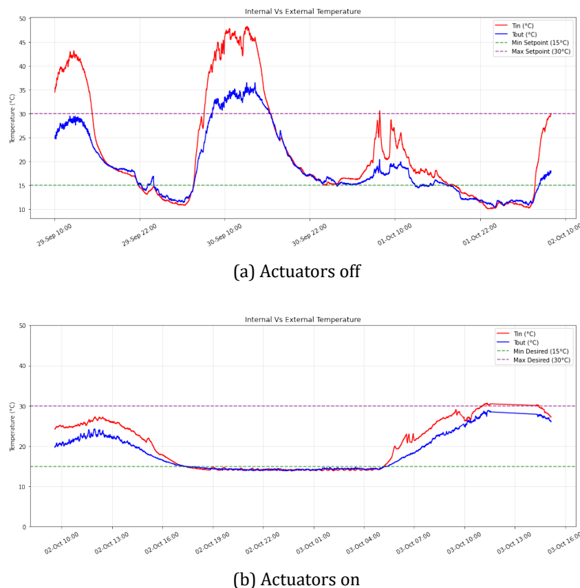
Figure 9.8: Internal vs. external temperature profiles for the greenhouse with (a) actuators off and (b) actuators on.
