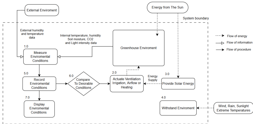
Figure 6.1: Functional decomposition
