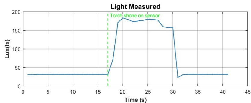
Figure 9.3: BH1750 light sensor response to torch illumination and return to ambient room lighting.
