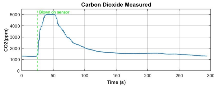
Figure 9.4: CO 2 sensor response
