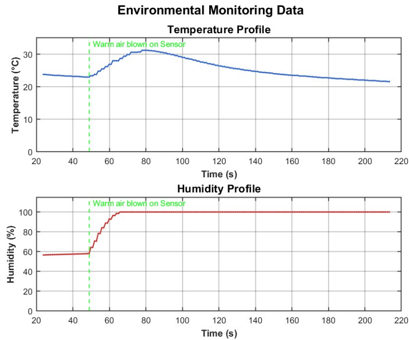
Figure 9.1: DHT22 response to applied warm air (temperature and humidity vs. time).
