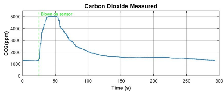
Figure 6.5: CO 2 sensor response to rapid change in concentration.
