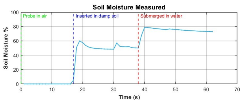
Figure 6.3: Soil moisture sensor response in open air, damp soil, and submerged in water.
