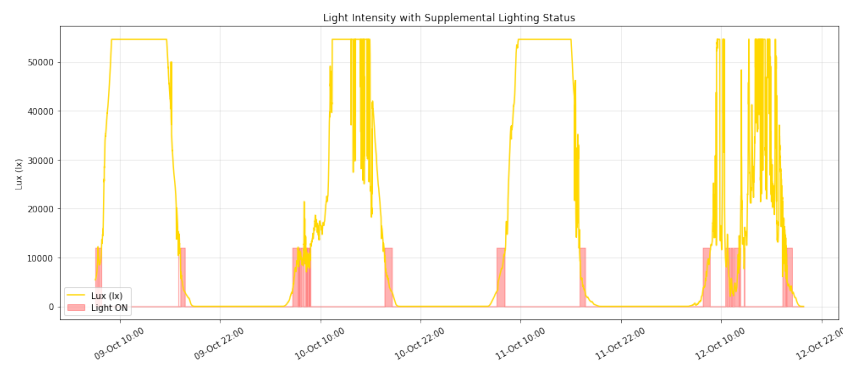
Figure 6.11: Lux Profile
