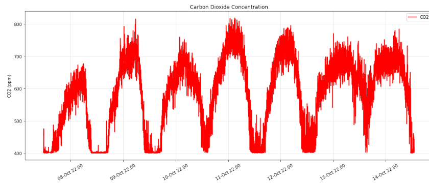
Figure 6.10: CO 2 Profile
