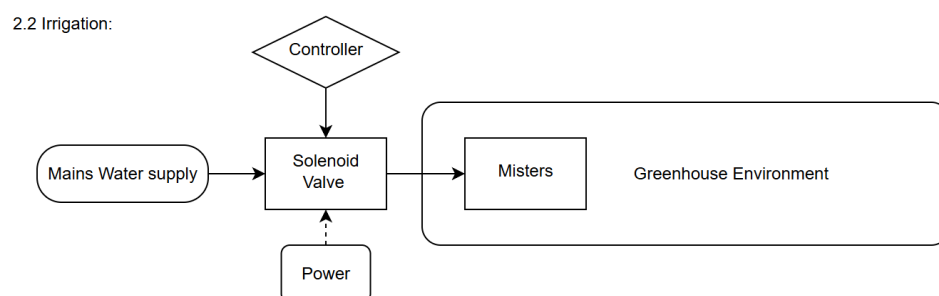
Figure 3.4: Irrigation Physical Decomposition
