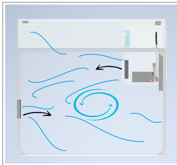
Figure 4.3: Air circulation
