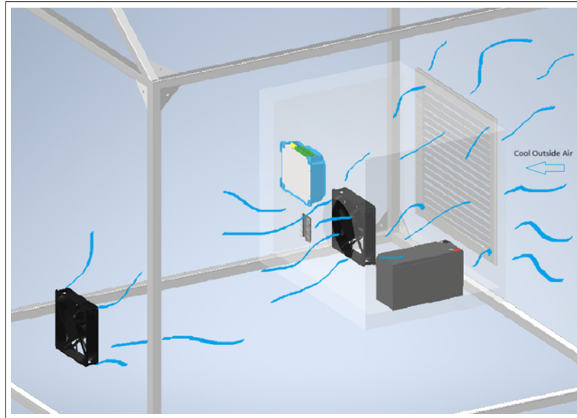
Figure 4.5: Air Intake
