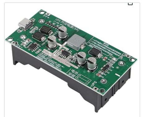
5 V UPS charger board.
