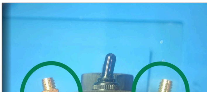
The two SMA bulkheads with the power switch centered between them.
