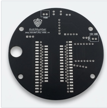
The bare 82 mm board.
