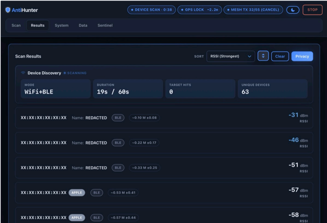
A device scan sending its results over the mesh. The header badge tracks the transmit queue draining at the LoRa airtime cap, 32 of 55 rows sent, and Privacy Mode has blanked the addresses.
