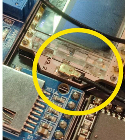
LoRa radio, socket circled.
