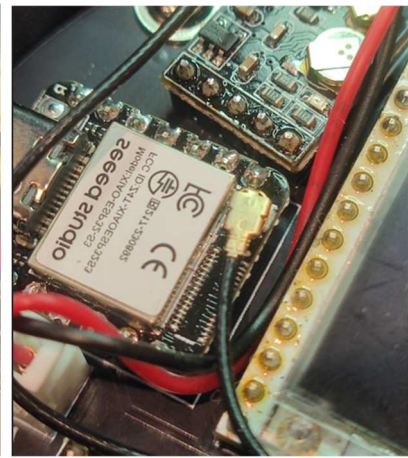
WiFi/BT Antenna
