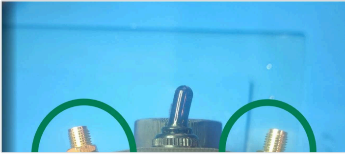
The two SMA bulkheads with the power switch centred between them.
