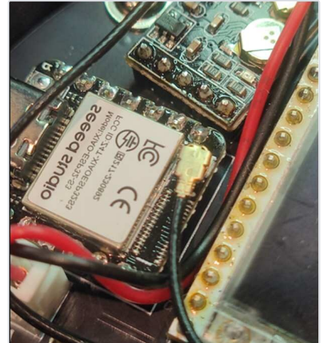
XIAO ESP32-S3, WiFi/BLE socket.
