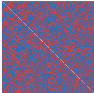
(a) PPSS, published order
