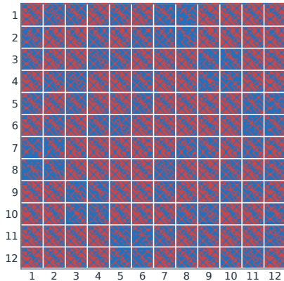
(b) Same graph, Clebsch order
