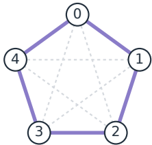
(a) Five labels in \mathbb{Z}_5
