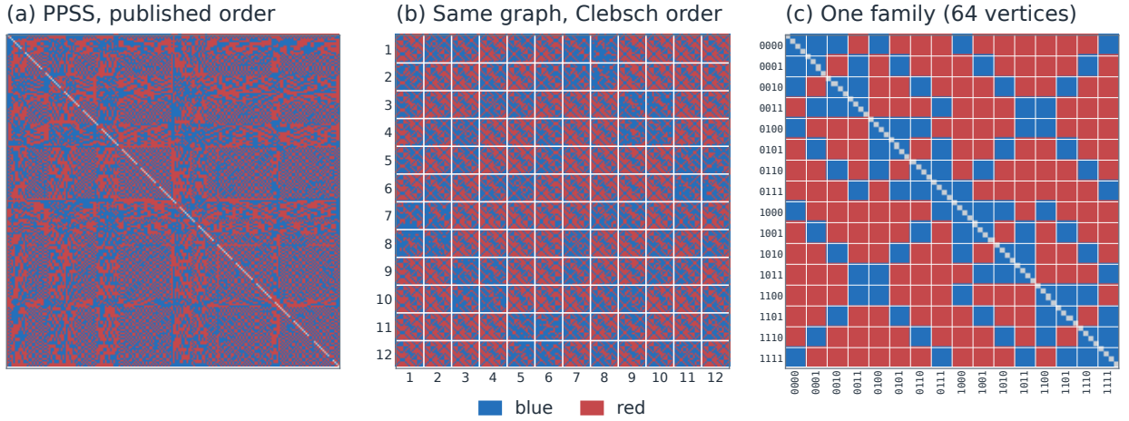
Figure 3: The PPSS graph [20] as a red/blue adjacency matrix. (a) In the published vertex order. (b) The same matrix with the vertices relabeled by Proposition 3.1: twelve families of 64 vertices. (c) One diagonal block: sixteen fibers of four vertices, colored by the Clebsch pattern of Figure 2(b). Gray marks the absent self-pairs.
