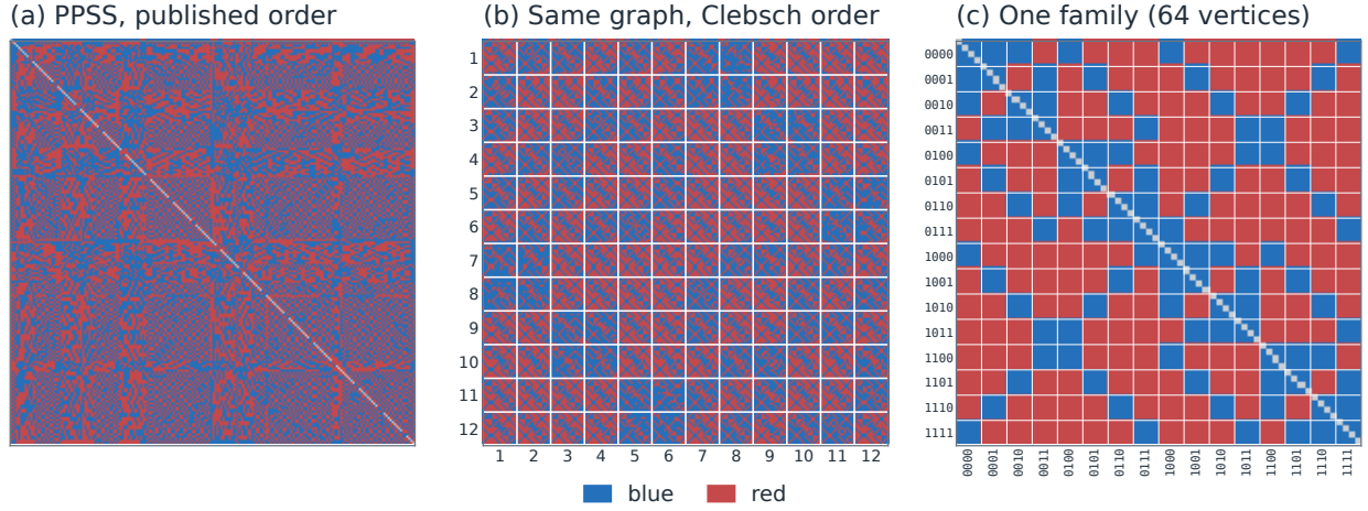
Figure 3: The PPSS graph [19] as a red/blue adjacency matrix. (a) In the published vertex order. (b) The same matrix with the vertices relabeled by Proposition 3.1: twelve families of 64 vertices. (c) One diagonal block: sixteen fibers of four vertices, colored by the Clebsch pattern of Figure 2(b). Gray marks the absent self-pairs.
