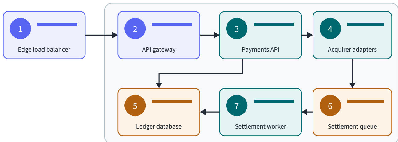
Figure 1. Request path through the production zone (shaded)
