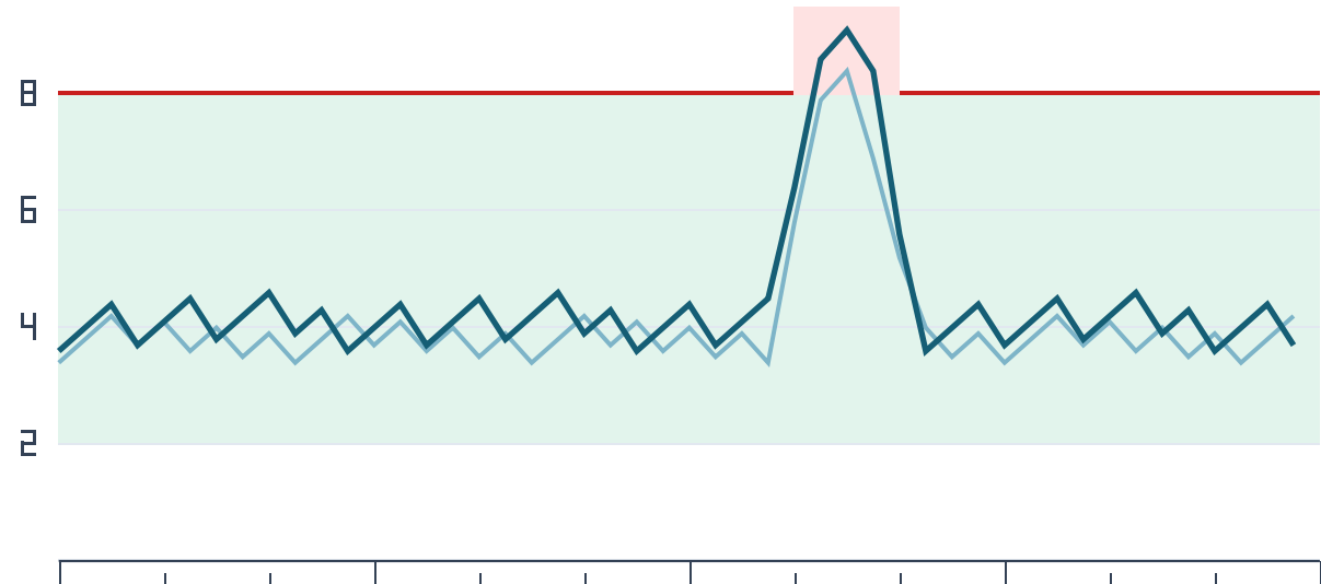
Figure 1. Probe A (dark) and probe B (light) against the 2 to 8 °C band; ticks every 2 hours from 06:00
