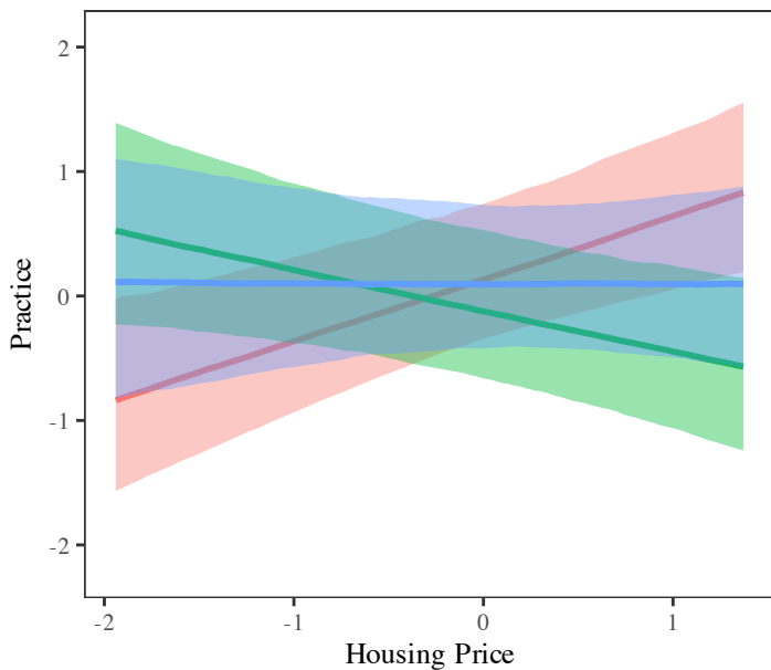
Model 3 (Test)
