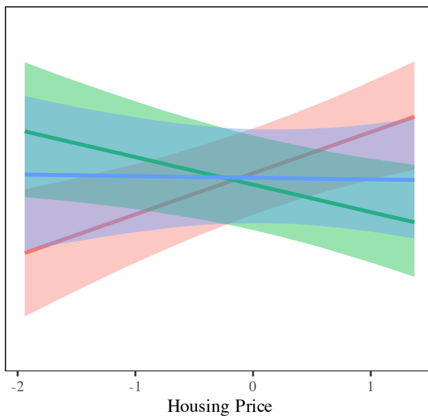
Model 3 (Joint)
