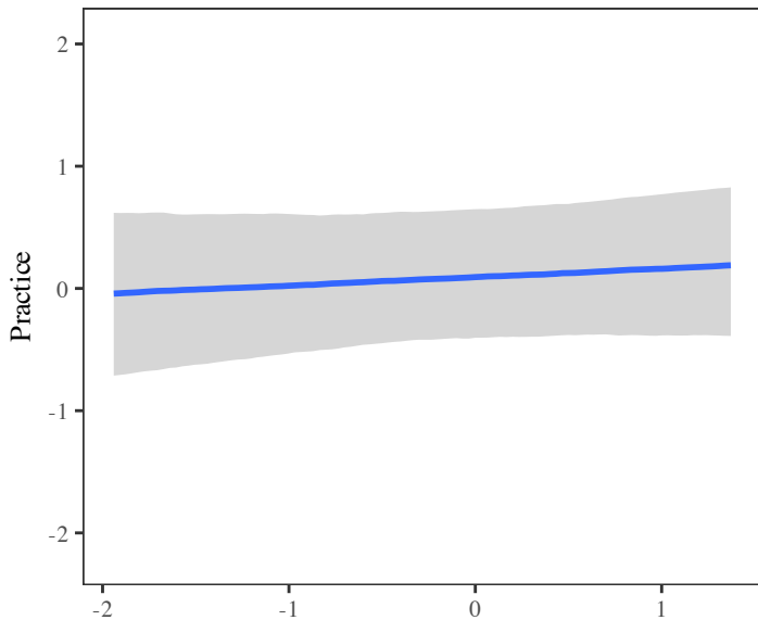
Model 3 (Test)
