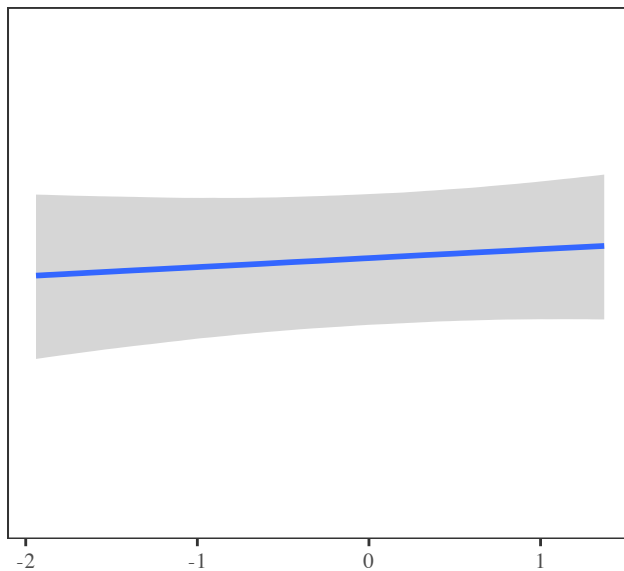
Model 3 (Joint)
