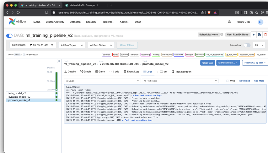
Figure 1: training phase
