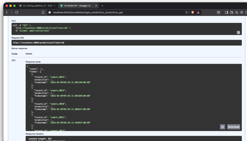
Figure 3: prediction results
