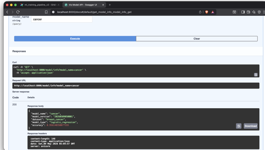
Figure 2: model info
