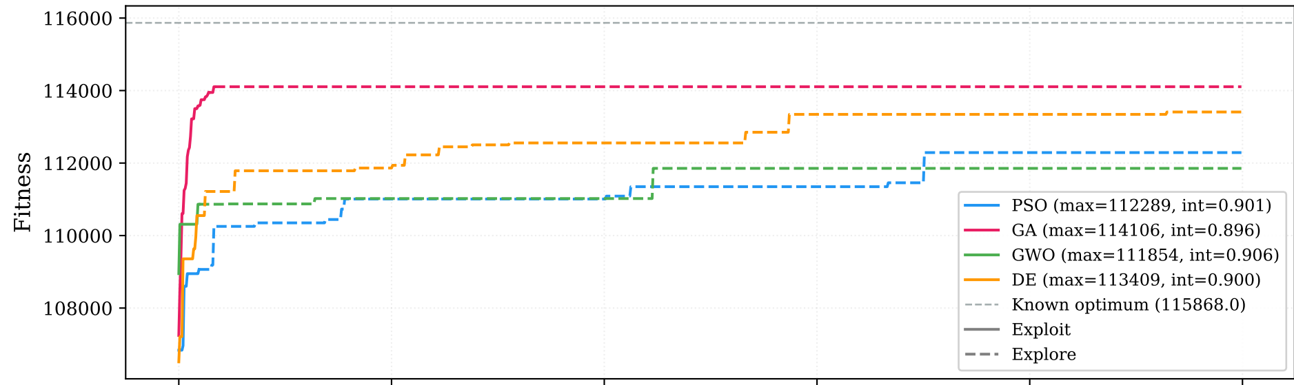
Continuous-Complex — All MHs (seed=1)
