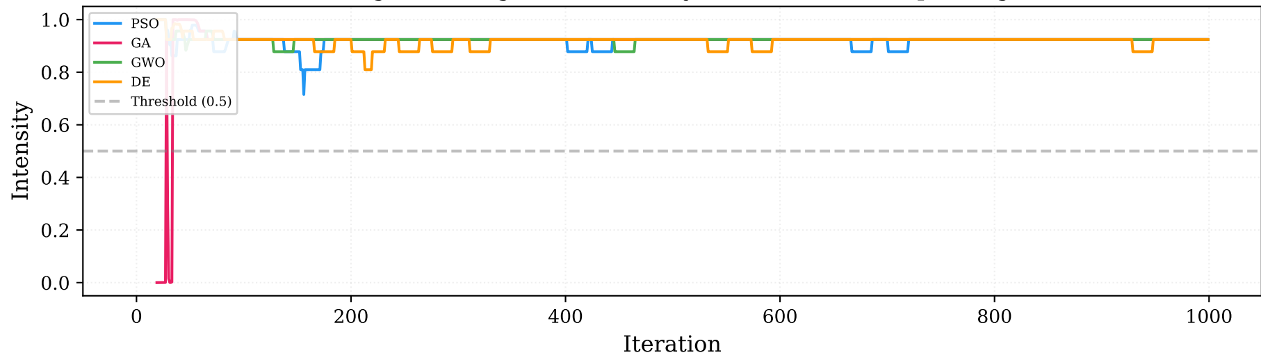
DTW Stagnation Signal — Intensity (Continuous-Complex sigmoid)
