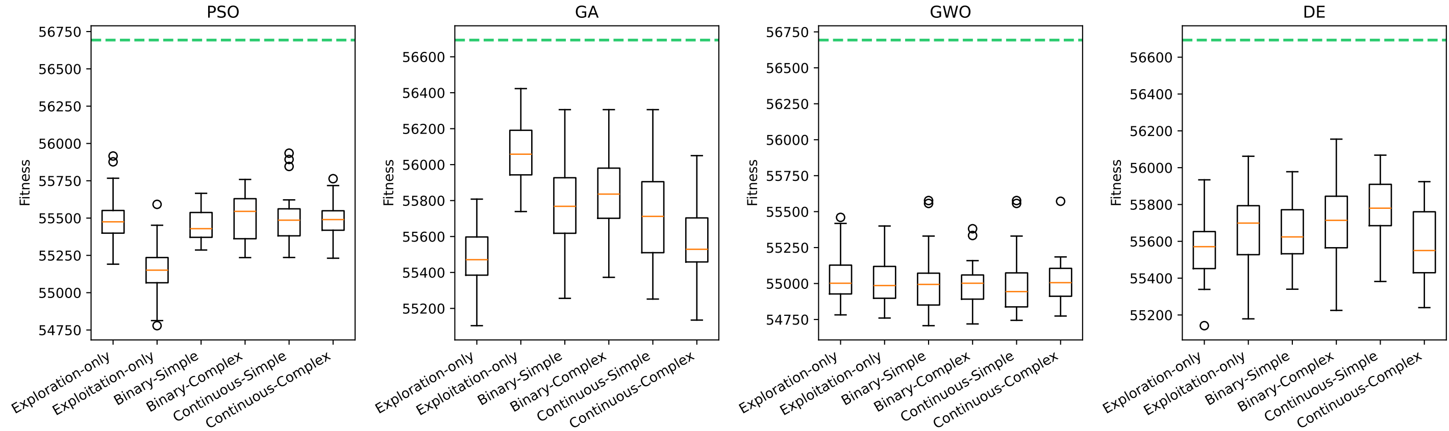
Fitness distribution across MH variants — mknapcb8[0] (opt=56693)
