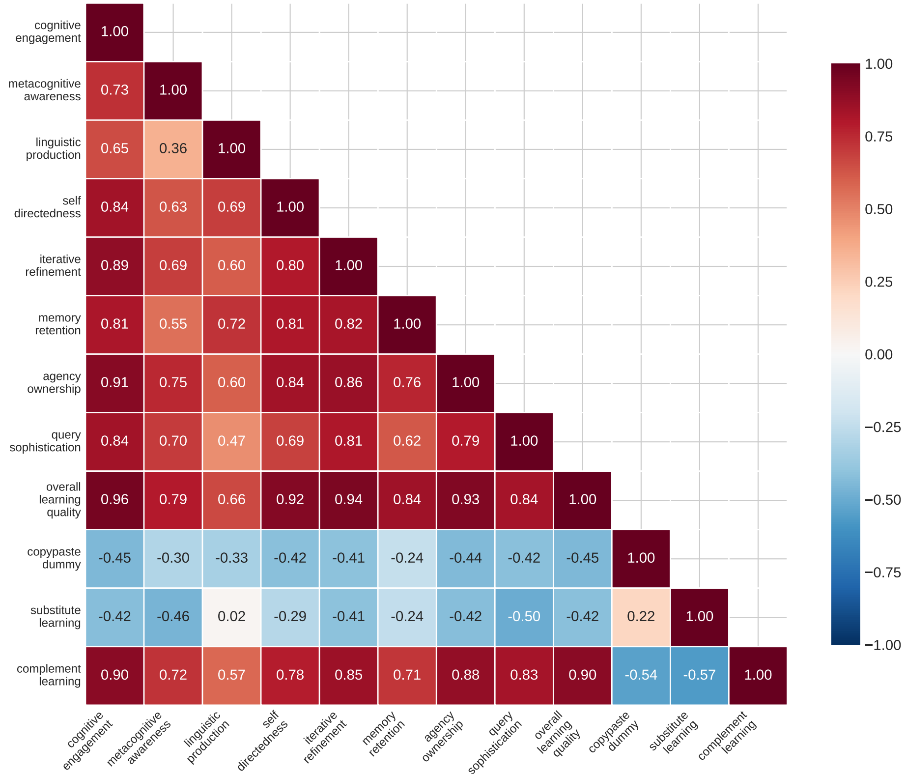
Metric Correlations (Explicit Evaluation)
