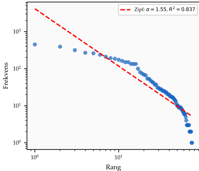
a) Zipf-plott (log-log)
