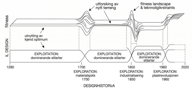
Fig. 10: Exploration/exploitation-dynamikk
