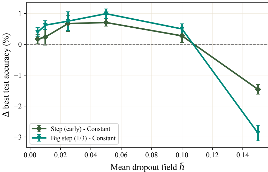
Scheduling advantage relative to constant dropout
