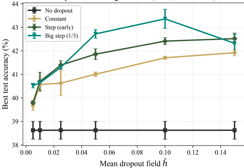
Dropout scheduling across \bar{h} (MLP, CIFAR-10)
