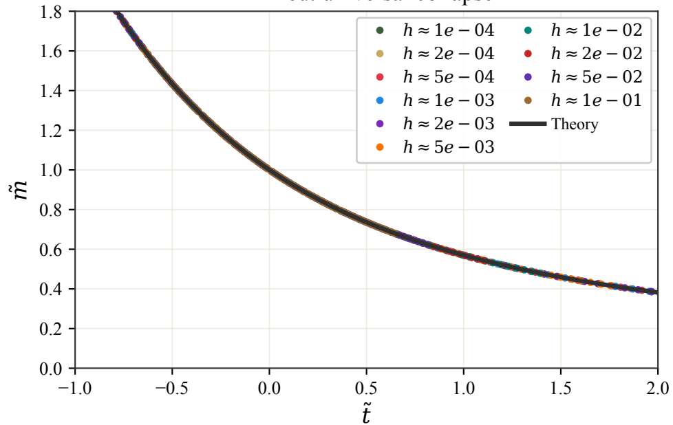
Kinked: universal collapse
