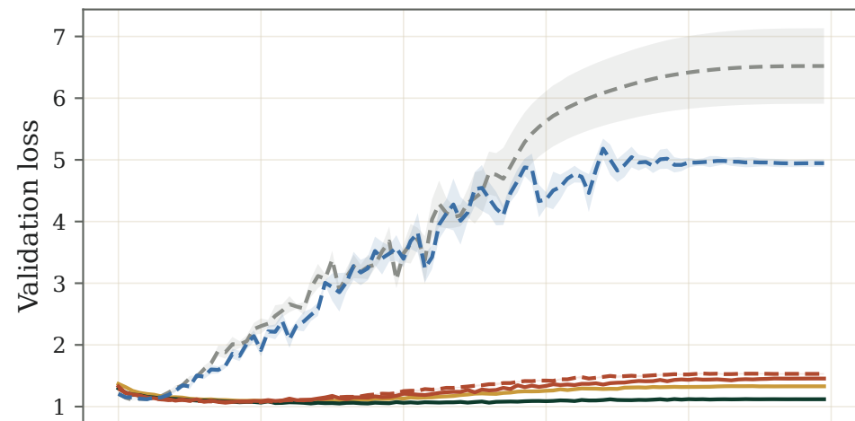
Validation loss
