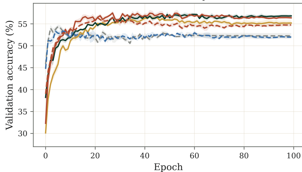
Validation accuracy (%)
