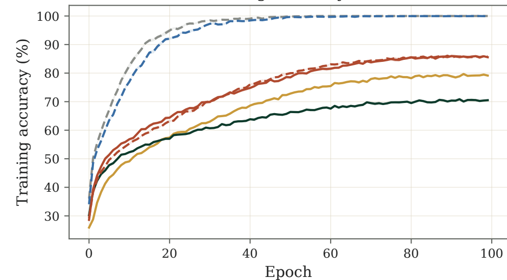
Training accuracy (%)
