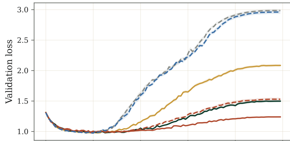
Validation loss
