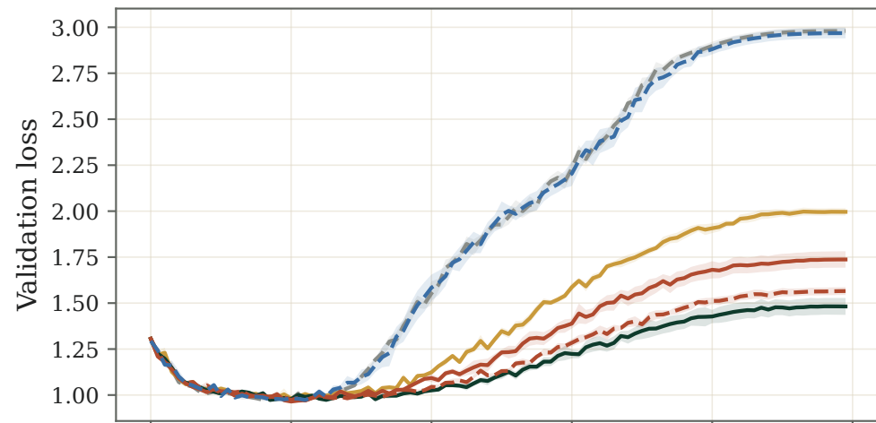
Validation loss
