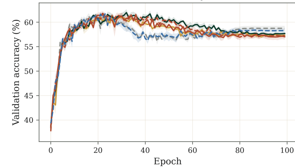
Validation accuracy (%)
