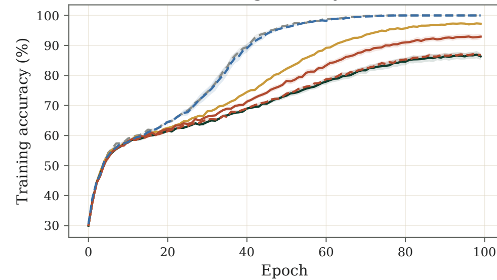
Training accuracy (%)
