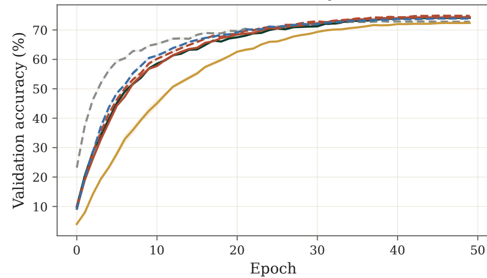
Validation accuracy (%)
