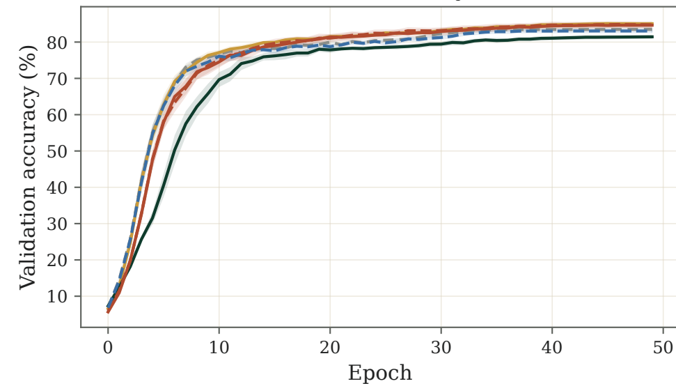
Validation accuracy (%)
