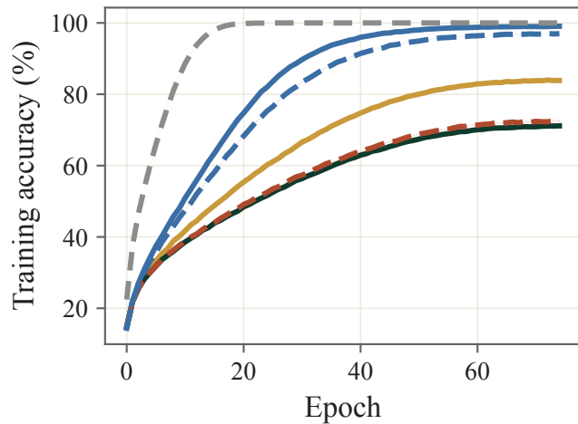
Training accuracy
