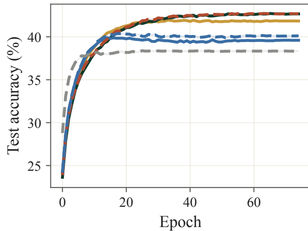
Test accuracy
