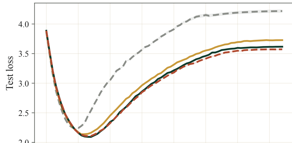
Test loss
