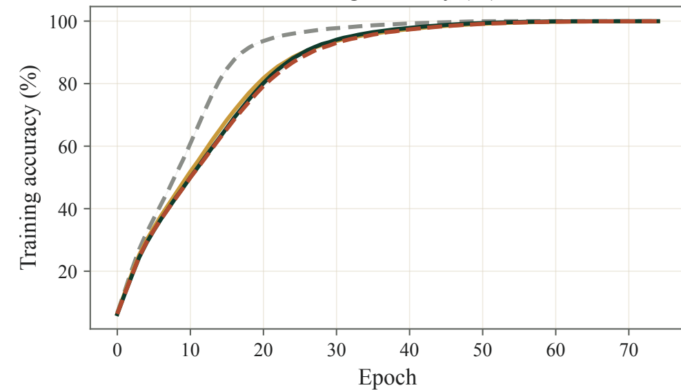
Training accuracy (%)
