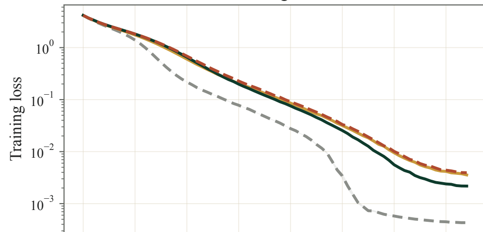
Training loss
