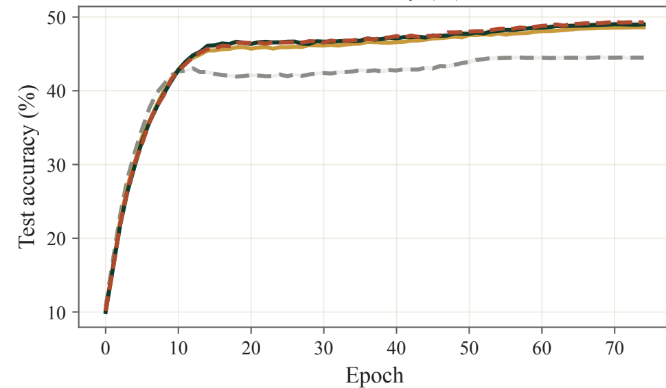
Test accuracy (%)
