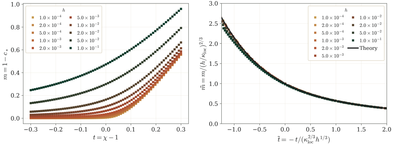
Figure 6. Kinked counterpart to Fig. 2. Each curve holds the field h fixed by setting \rho = \chi/(\chi + h) in the formal ReLU channel above. The points solve the full map; rescaling uses its local kink coefficient \kappa_{\text{loc}} = \chi 2\sqrt{2}/(3\pi) . The horizontal coordinate reverses the sign of u in Eq. (38), evaluated with this coefficient, which approaches the critical value as \chi \rightarrow 1 . The black curve is the leading equation of state, and the remaining departures at larger fields come from higher-order terms. This formal comparison does not require independently tunable finite-variance ReLU initializations.
