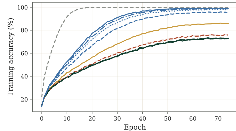
Training accuracy (%)
