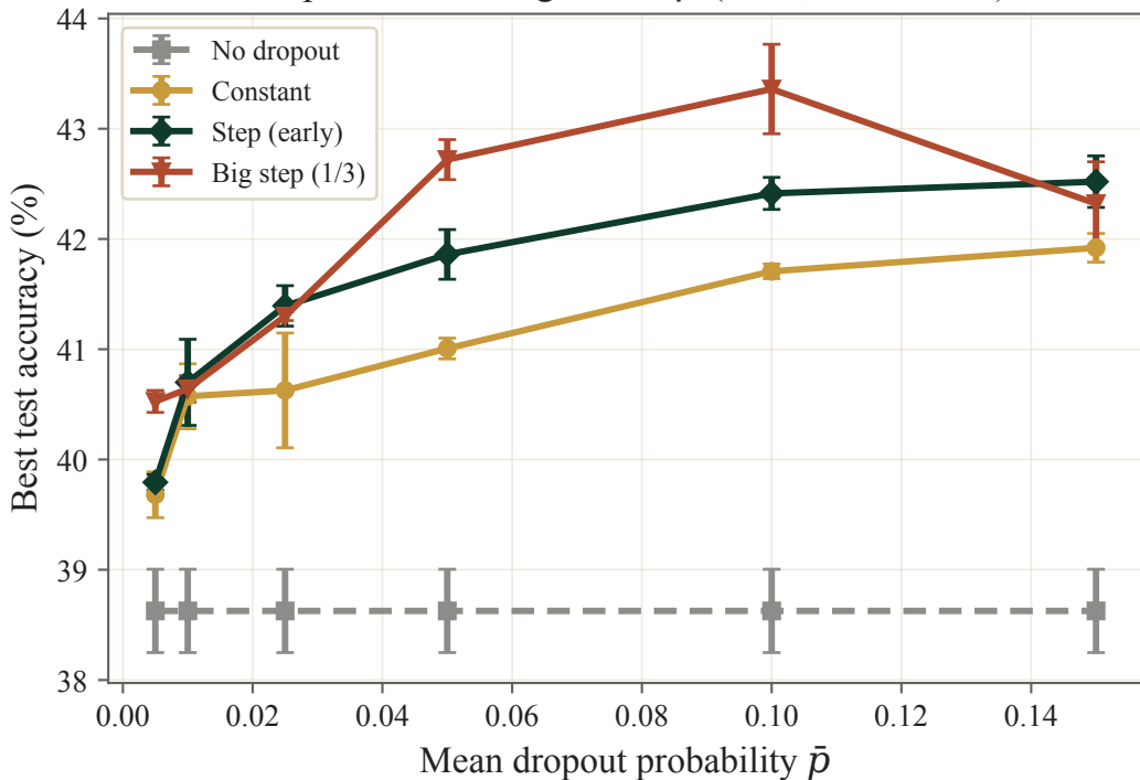
Dropout scheduling across \bar{p} (MLP, CIFAR-10)
