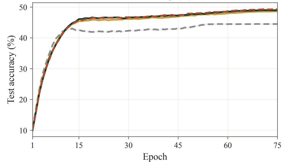
Test accuracy (%)
