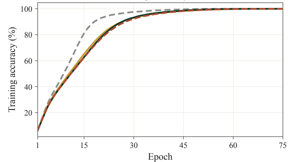
Training accuracy (%)
