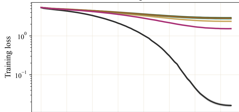
Training loss
