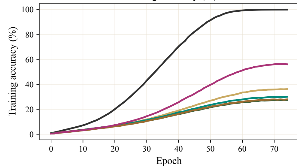
Training accuracy (%)
