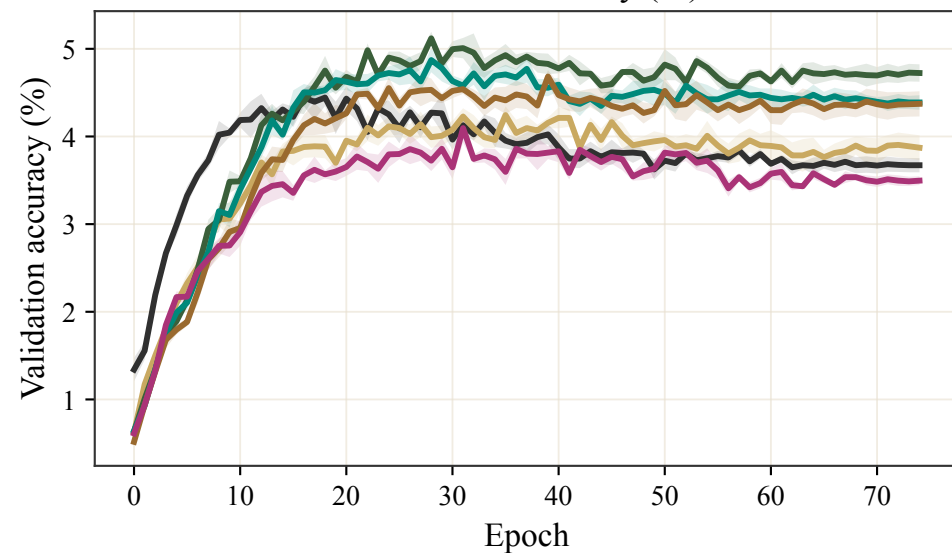
Validation accuracy (%)
